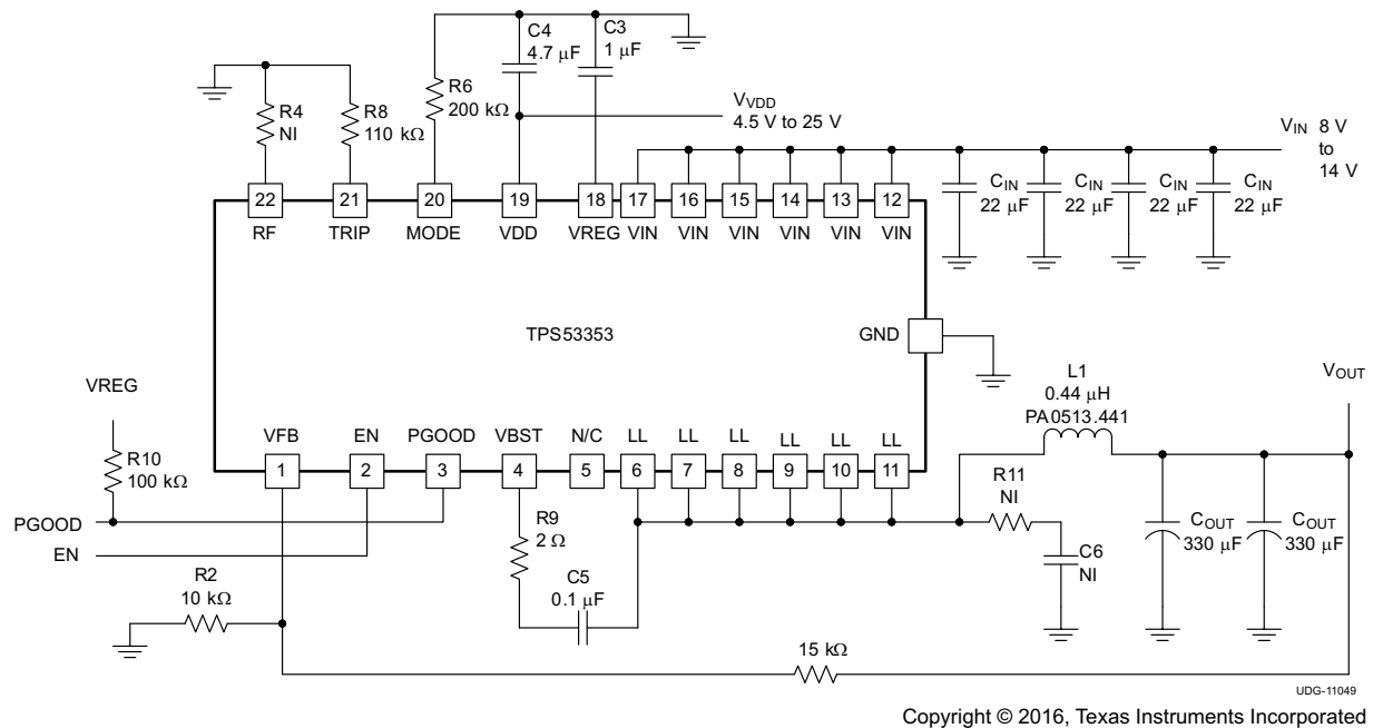
8-1. Typical Application Circuit Diagram
