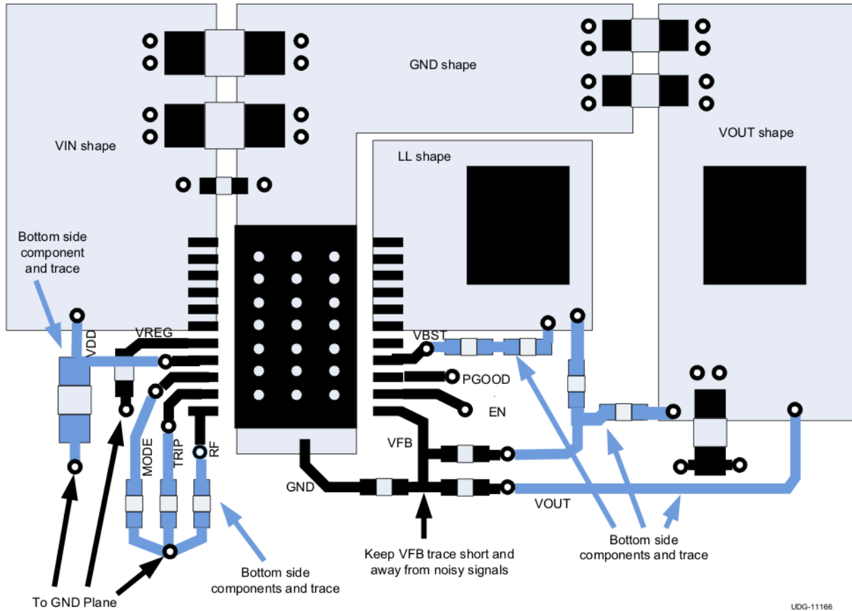
☒ 10-1. Layout Recommendation
